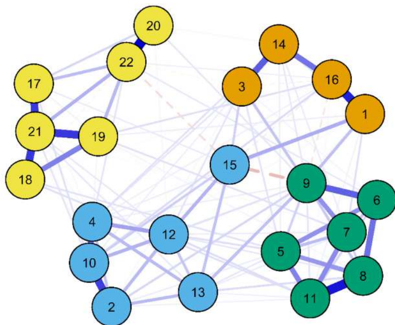
Fig. 1. Network visualizations.
